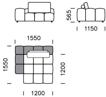
Left seat 1
